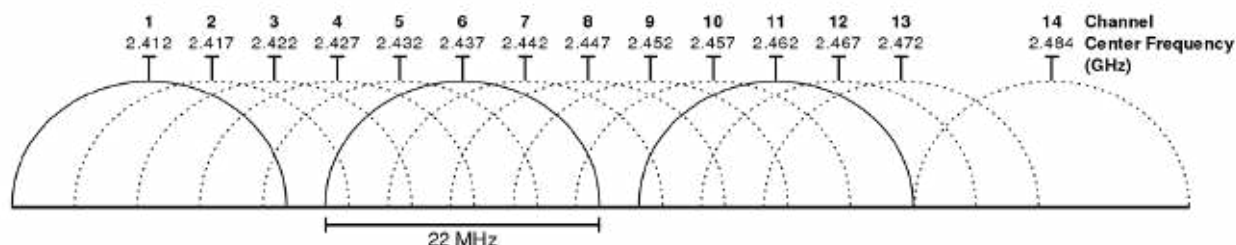
Figure 15 - 2.4 GHz Wi-Fi channels 26
